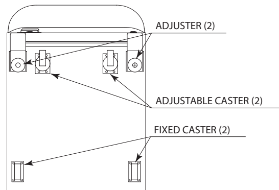
FIG. 6.1a Bottom View
