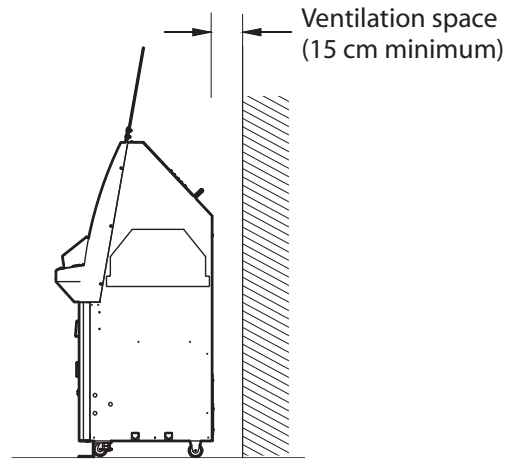
FIG. 6.1e Ensuring Ventilation Space
